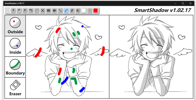
Fig. 1. Screenshot of the SmartShadow. The user gives scribbles as shadow indications (on the left) to obtain the high-quality shadow (on the right). Smiling boy, used with artist permission.
