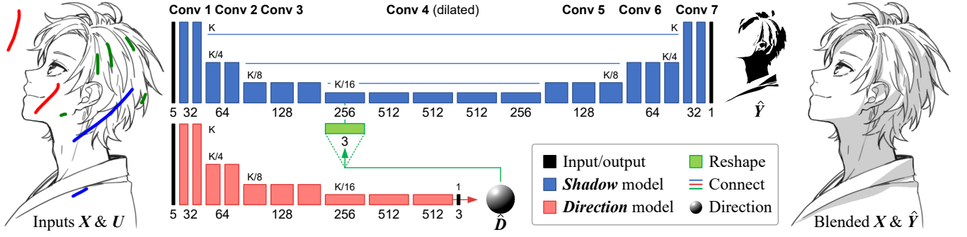
Fig. 3. Network architecture. We train two branches of the shadow drawing network. Both branches use the blue layers for predicting the shadow. The direction model branch uses red layers for predicting the global shadow direction. The shadow model branch uses blue layers for predicting the final output shadow. All convolutional layers use 3 \times 3 px kernels. We do not use any normalization layers. Shortcut connections are added to upsampling convolution layers. Boy looking upside, used with artist permission.
