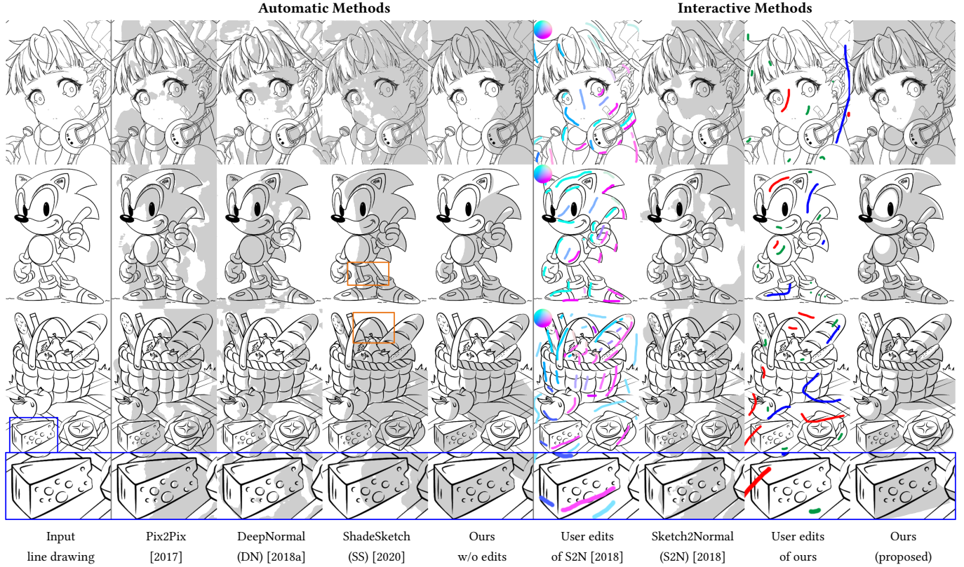
Fig. 6. Comparisons to possible alternative methods. 15 more full-resolution comparisons are provided in the supplementary material. The user scribbles are precisely one-pixel width and we dilated the scribbles for clearer presentation. Artworks used with artist permissions.
