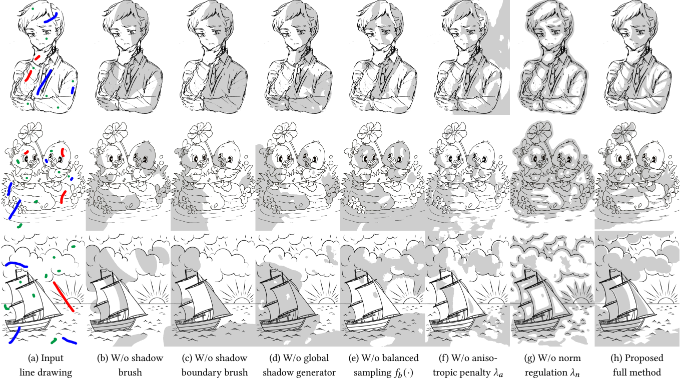
Fig. 7. Ablative study. We study the impact of each individual component within our framework by removing components one-by-one. The user scribbles are precisely one-pixel width and we dilated the scribbles for clearer presentation. Artworks used with artist permissions.
